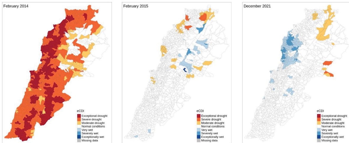
Maps produced by the enhanced Composite Drought Index (eCDI) showing drought and wet conditions in Lebanon. Source: Maps created by Karim Bergaoui, IWMI.
